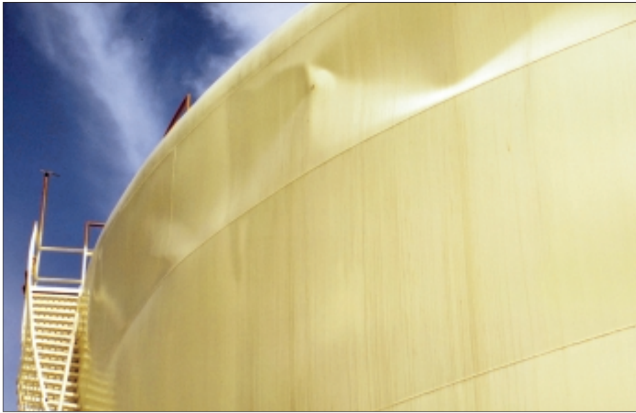
Fig. 2: Sloshing damage to upper shell of tank (courtesy of University of California at Berkeley)
